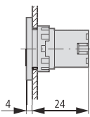
Q...BS
